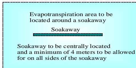
Location of evapotranspiration area on level land
