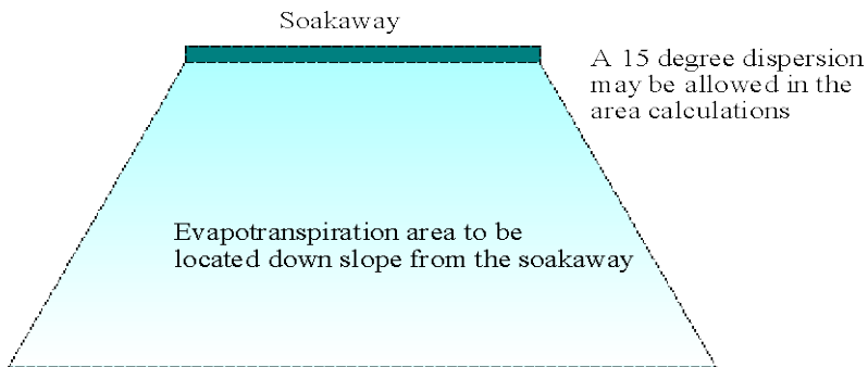
Location of evapotranspiration area on planar slope
